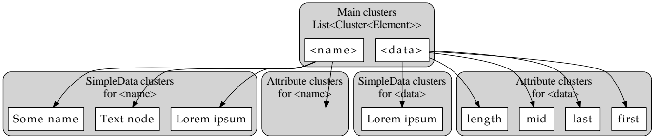
Figure 3: Iname clusterer structure
