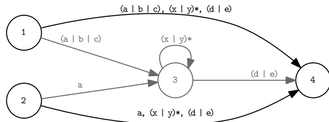
(d) Bypass state 3 by adding concatenation transitions from states 1 and 2 to state 4. Remove state 3 and associated transitions.
