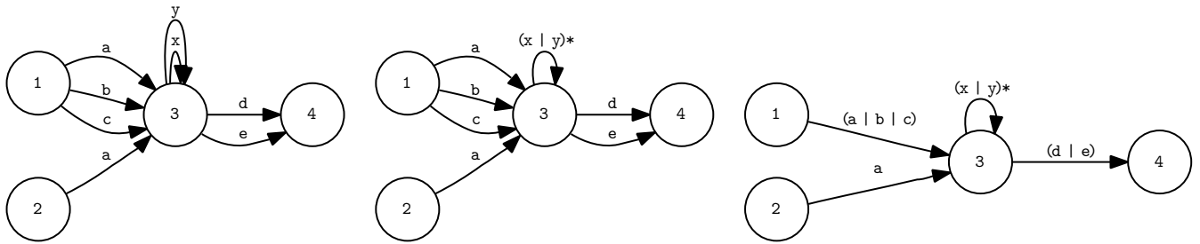
(a) RegexpAutomaton after conversion from ordinary automaton. (b) First, collapse loop transitions to alternation with Kleene interval set. (c) Collapse in- and out-transitions from state 3 to same states.
