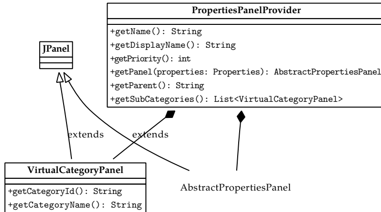
Figure 3: Class diagram for the custom jInfer project properties category.
