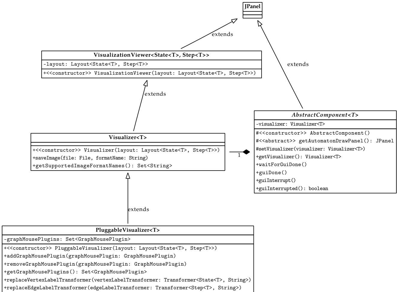
Figure 1: Class diagram for the base classes.
